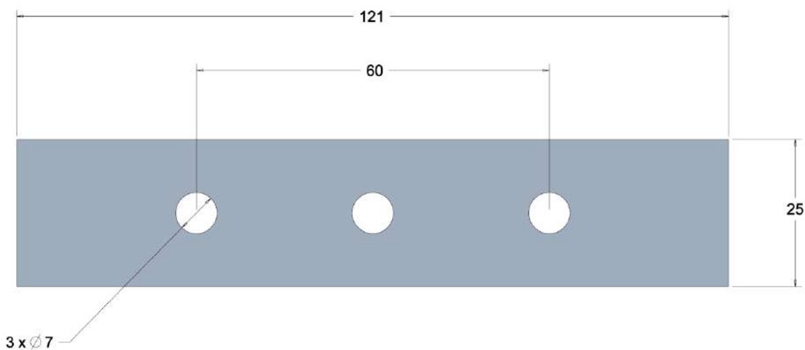
Mounting Holes
