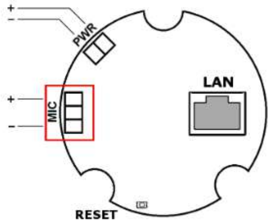
Non-symmetrical microphone
