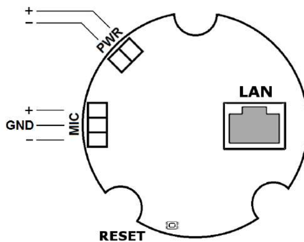
2N® SIP Speaker Horn back panel
