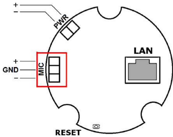
Symmetrical microphone
